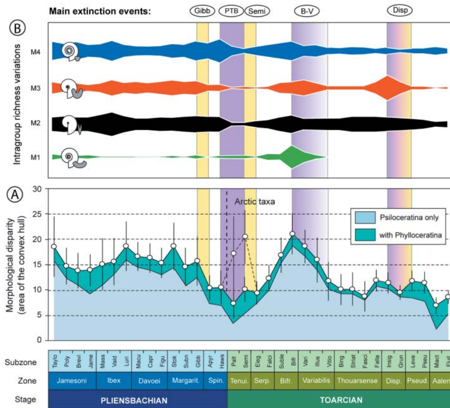
Fig. 8. Impacts of the five main extinction events on the morphological patterns.
