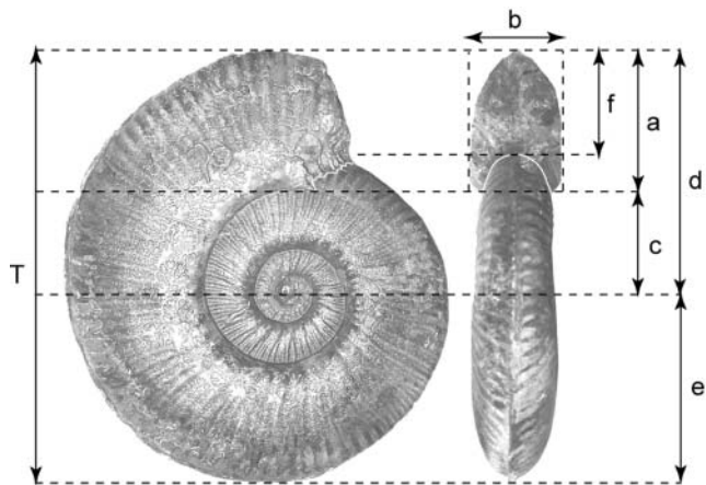
Fig. 3. Morphometric measurements of ammonite shells. The five derived shape ratios used in this study are: D = c/d ; S = b/a ; W = (d/e)^2 ; RW = b/T ; AH = f/a .
