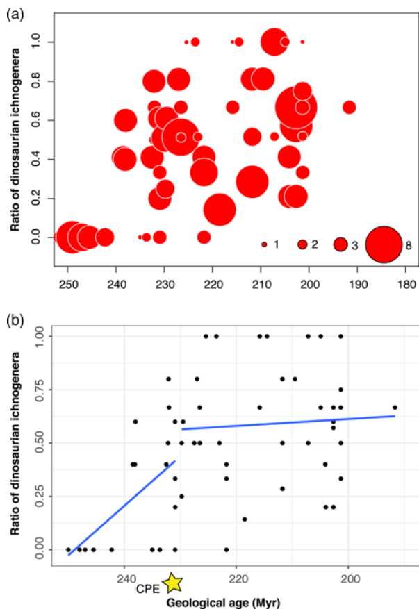
Fig. 5. Relative proportions of dinosaur to other archosaur footprints through the Triassic, focusing on Late Triassic ichnoassociations, shown as a bubble plot of ichnofaunas and their sizes (a), and as dated points with suggested break point indicated (b). Values jump from essentially no, or very rare, dinosaurs, before 232 Ma, corresponding to the CPE, and then mean values of 48% in the late Carnian, 56% in the Norian and 70% in the Rhaetian. Formula for pre-CPE line is y = 0.0179x + 4.4718 ( R^2 = 0.27 ), and for post-CPE line is y = 0.0033x + 1.291 ( R^2 = 0.02 ). (Based on data in supplementary material Table S3.)
